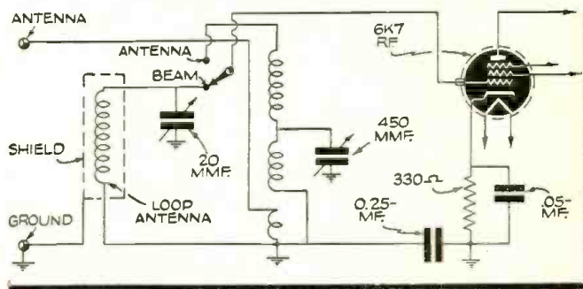
Hook-up of "Beam-O-Scope." No. 1160.
